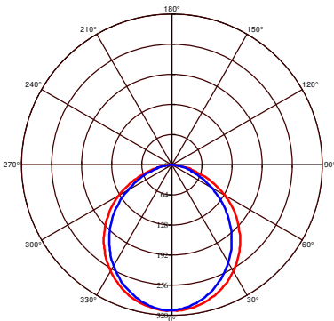
b C0 Plane beam angle(50%) b C90 Plane beam angle(50%) C0 Plane beam angle(50%):109.5(DEG) C90 Plane beam angle(50%):39.1(DEG)
