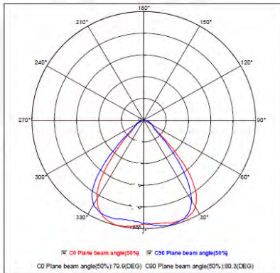
Planar Intensity Distribution Curve
